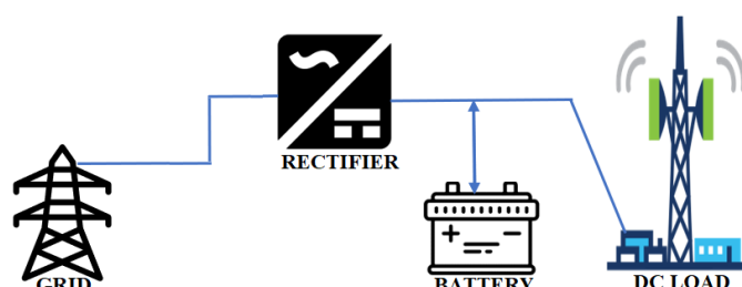
Figure 10.3.1 System block diagram of DC power system
