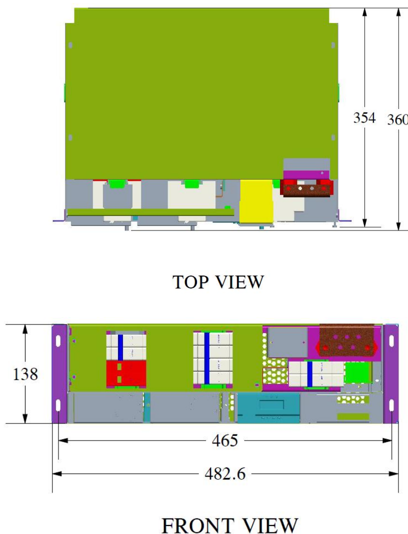
Figure 9.1 Dimension of Full system Figure
