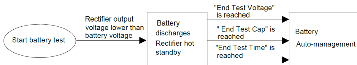
Fig 11.10.1 Testing function operating principles
