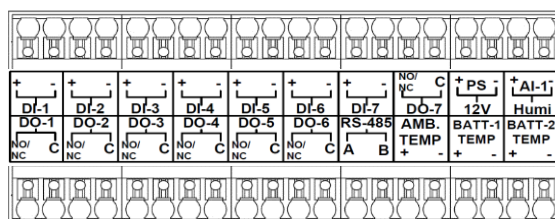
Figure 10.10.1 user interface board front panel
