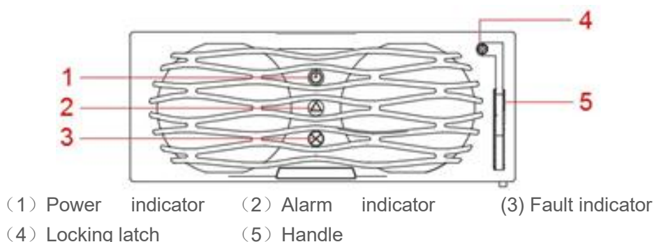
Figure 10.8.1 Rectifier panel
