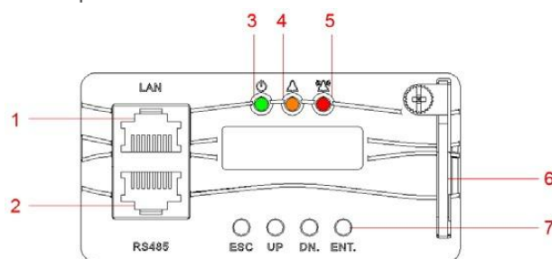
Figure 10.9.2 Front panel of the monitor module
