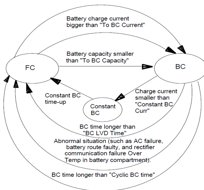
Fig 11.8.1 The BC/FC switchover diagram
